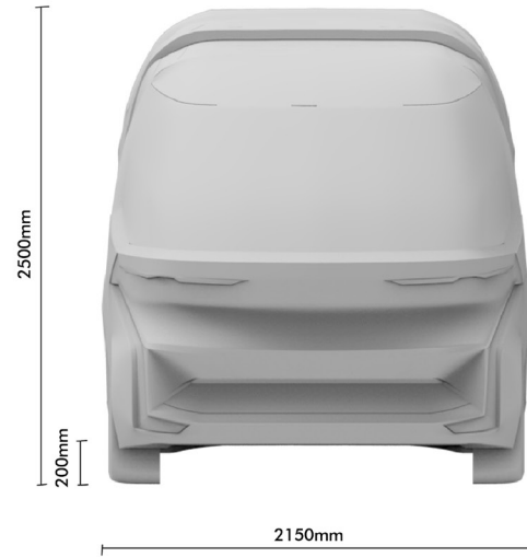
Image 23.1 Vehicle Dimension and comparison with Lexus LS500h
