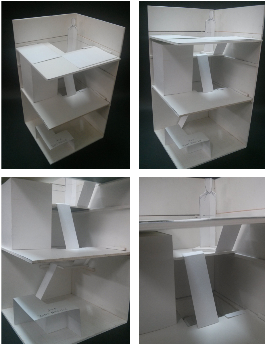
Fig 19. Foam board mockup (in clock-wise from top-left) 1.Full model ; 2.Toilet space at level 1; 3.Kitchen space at level 0; 4.Height clearance.
