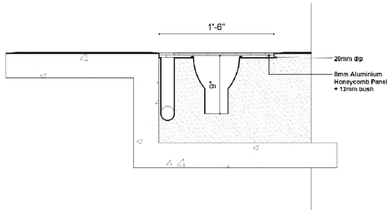
Fig 47. Commode, commode lid and floor trap details
