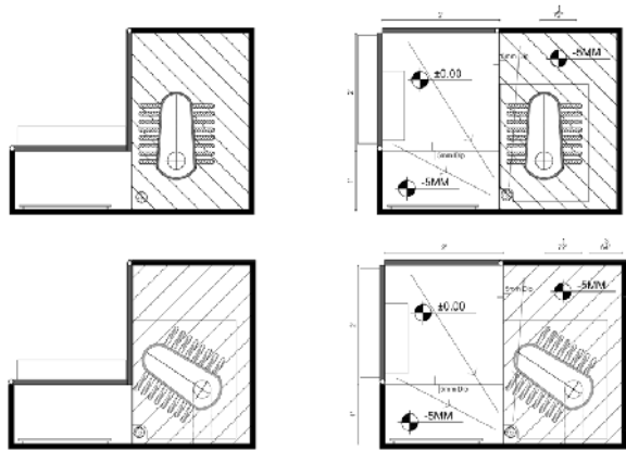
Fig 43. Toilet pan details of alternative 2
