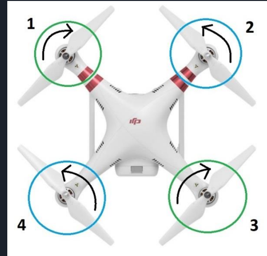
Rotational directions on quadcopters
