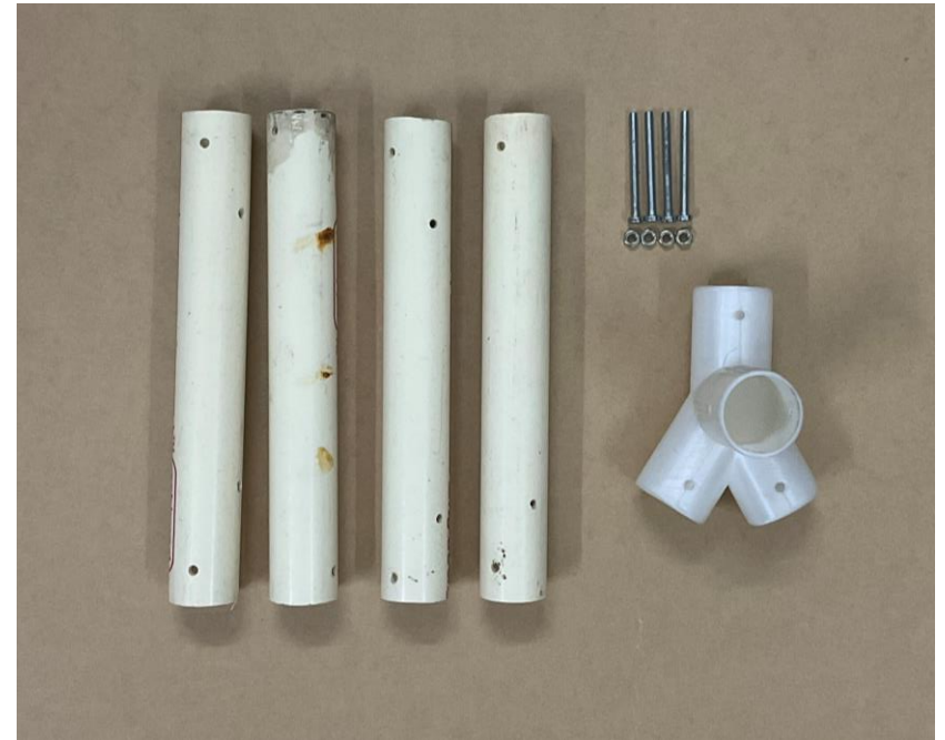
Fig.58.2 Mockup 4- joinery 1
