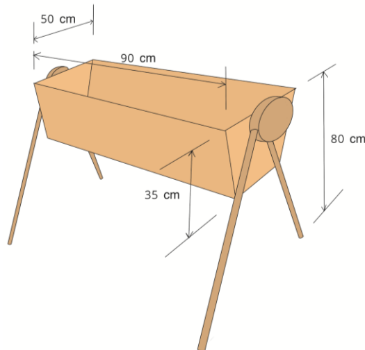
Fig.40 Dimensions for cradle
