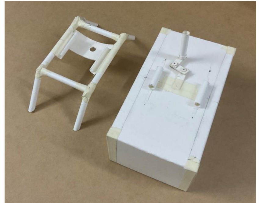
Fig.56.2 Mockup 2- idea 6
