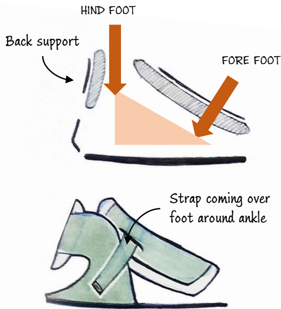
FIG. 9.1 REQUIRED FASTENING FOR FOOT
