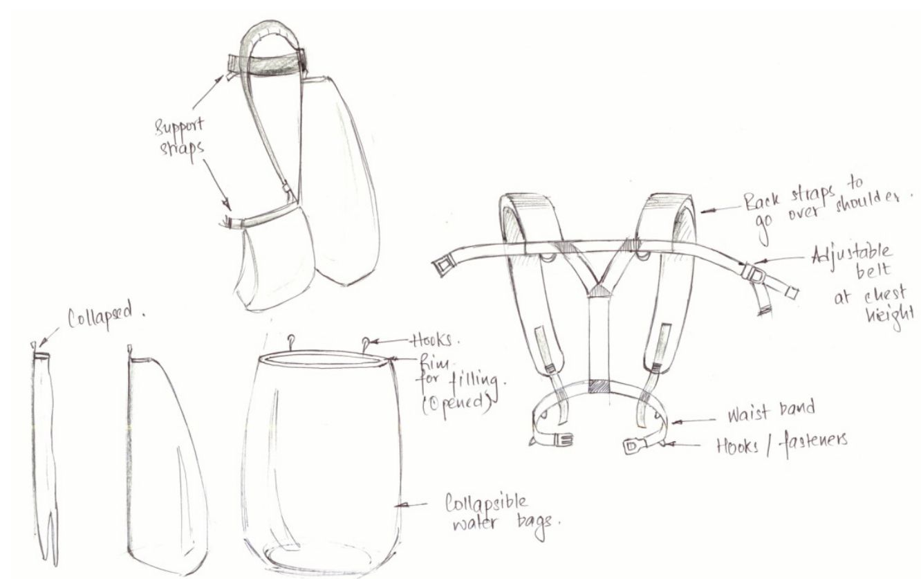
Fig 1: Vest design for water bags
