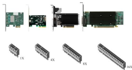
Figure17 : PCI express card and slot configuration
