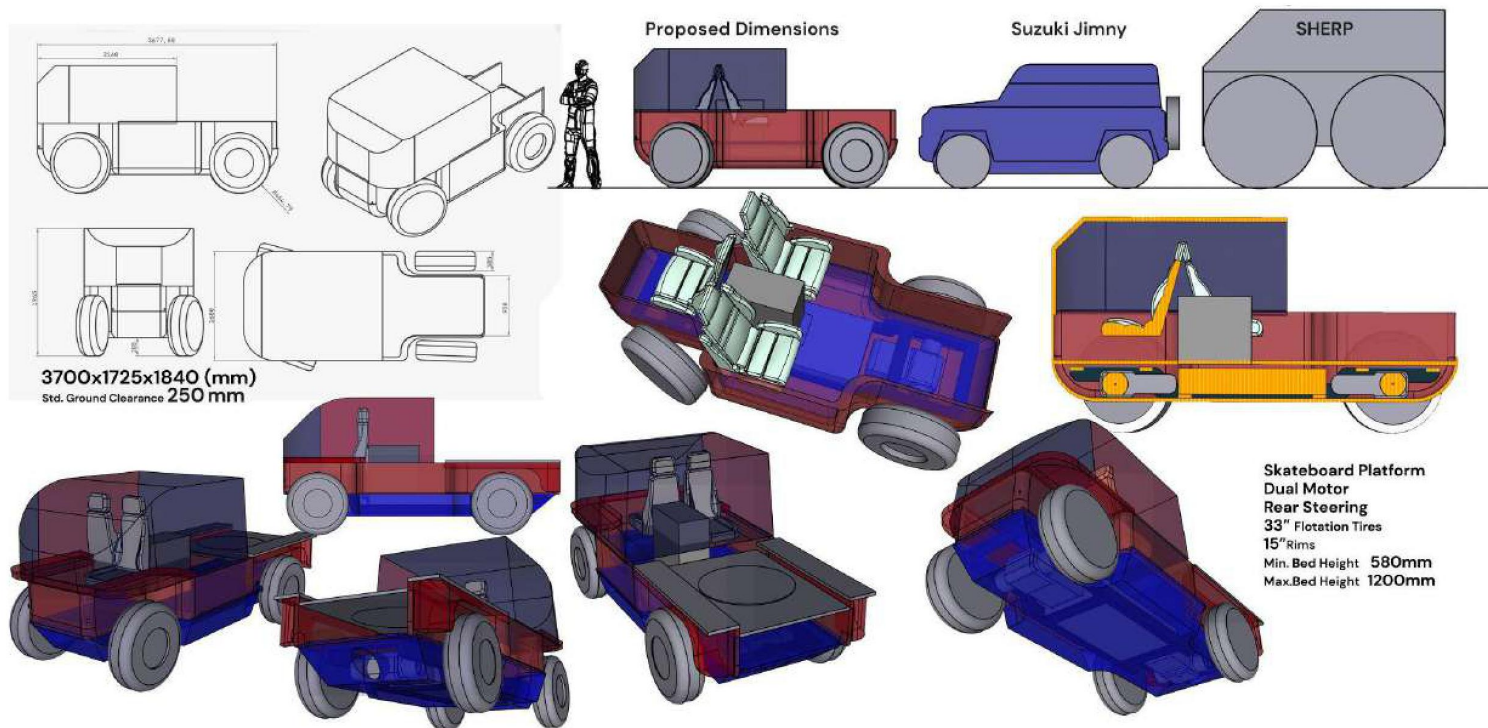
Fig. 11a Initial platform exploration in CAD
